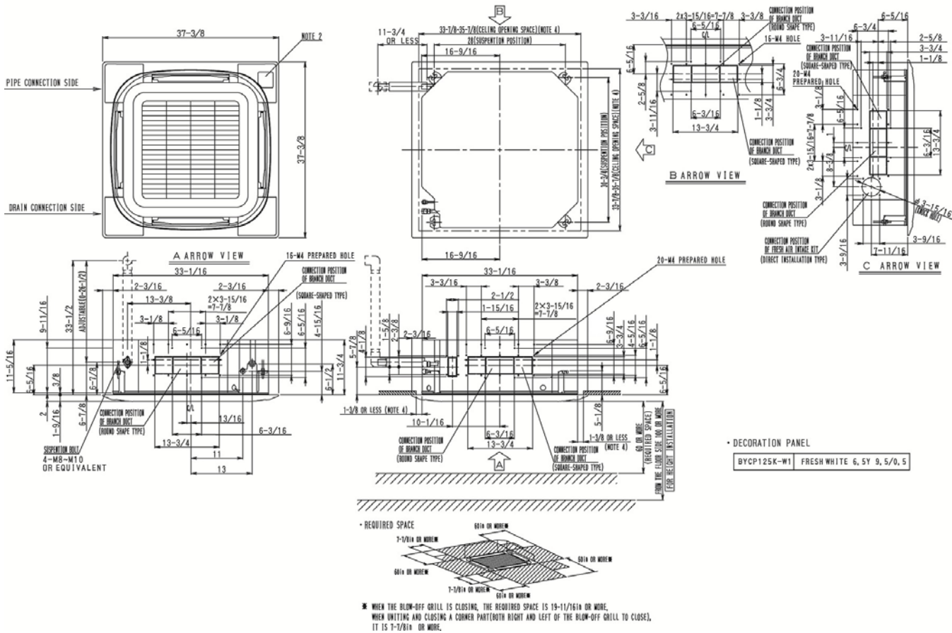
FXFQ36/48PVJU Unit (inches)
